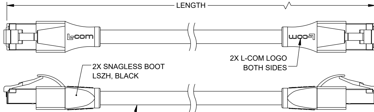
CAT 7 SHIELDED MODULAR CABLE FOUR TWISTED PAIR WITH ALUMINUM/ POLYESTER FOIL SHIELDING OF EACH PAIR CONDUCTORS: 26 AWG STRANDED COPPER OVERALL SHIELD: TINNED COPPER BRAID JACKET: LOW SMOKE ZERO HALOGEN, COLOR: RED, NOM. DIA. .236 [6] (OPERATING TEMPERATURE: -10°C TO +80°C; VOLTAGE RATING: 30V)
